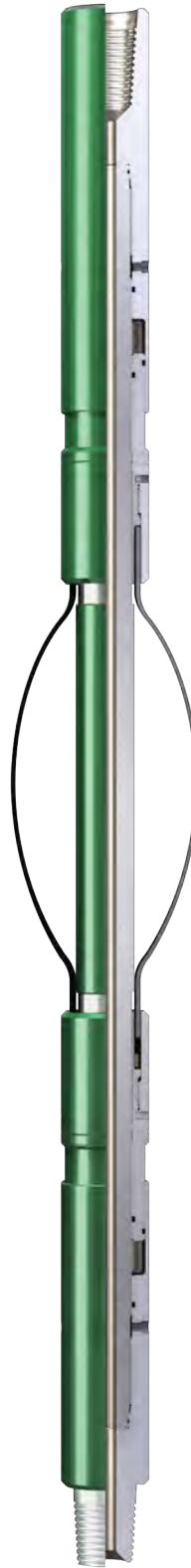
Hydraulic bowspring centralizer
