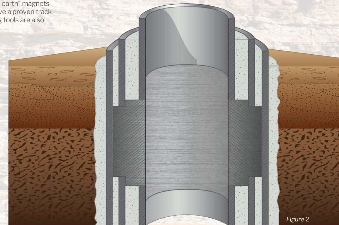
Figure 2: Barrier in place and wellbore access re-established.
