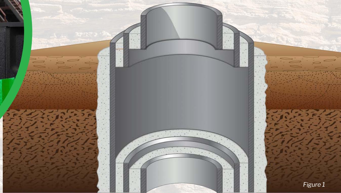
Figure 1: Preparation of zone prior to barrier installation.
