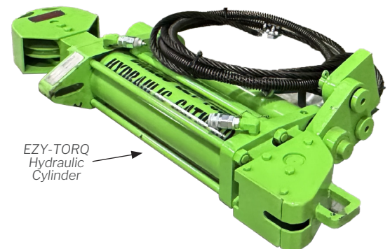
EZY-TORQ Type SC Power Unit System
